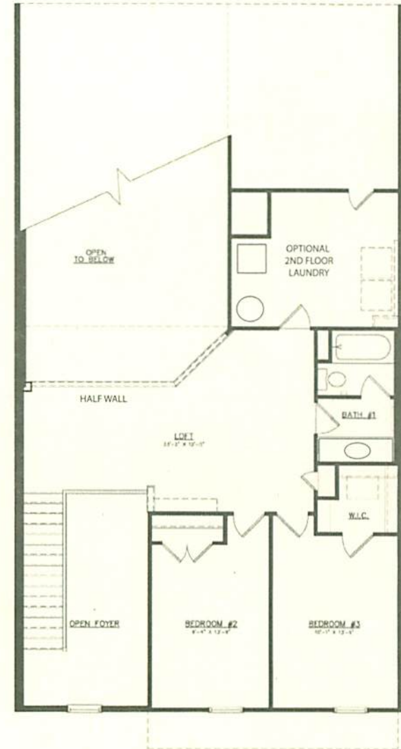
SECOND FLOOR
