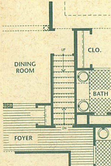
PARTIAL FIRST FLOOR PLAN OPTIONAL BASEMENT ENTRANCE
