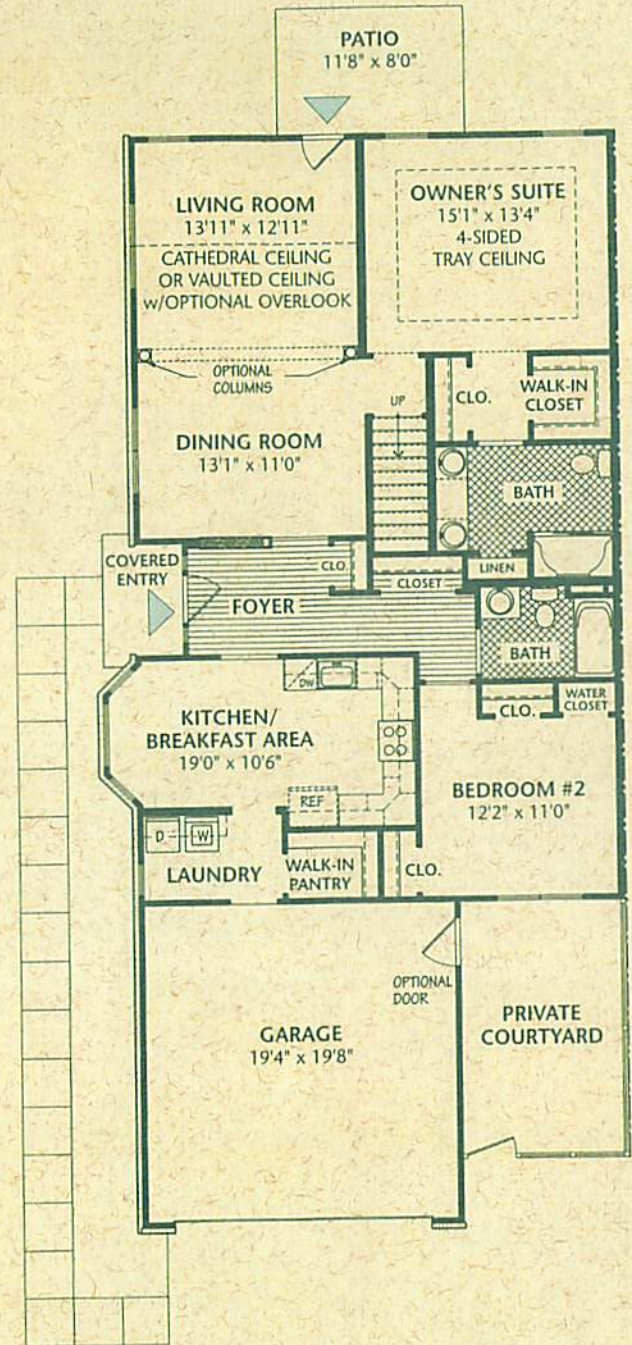
FIRST FLOOR PLAN 9'-0" FIRST FLOOR CEILINGS
