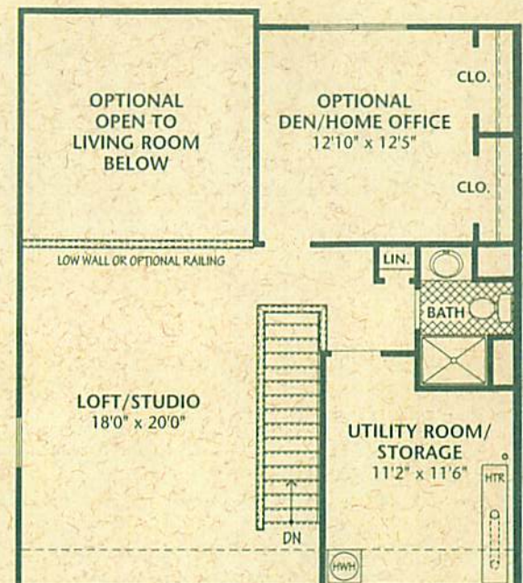
OPTIONAL FINISHED LOFT/STUDIO SHOWN w/OPTIONAL OVERLOOK, OPTIONAL BATHROOM & OPTIONAL DEN/HOME OFFICE
