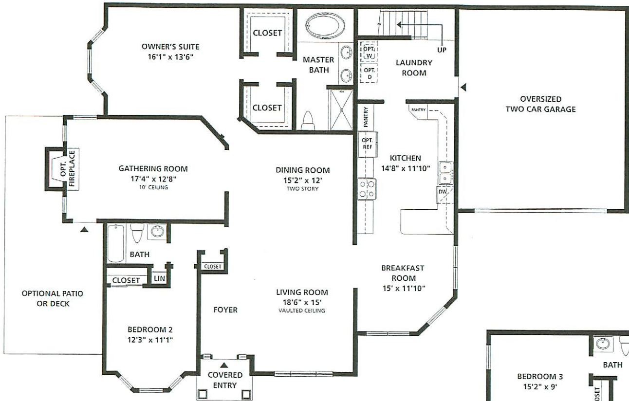
FIRST FLOOR
