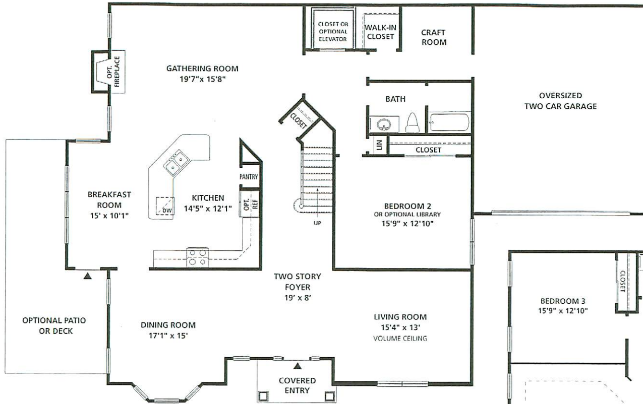
FIRST FLOOR
