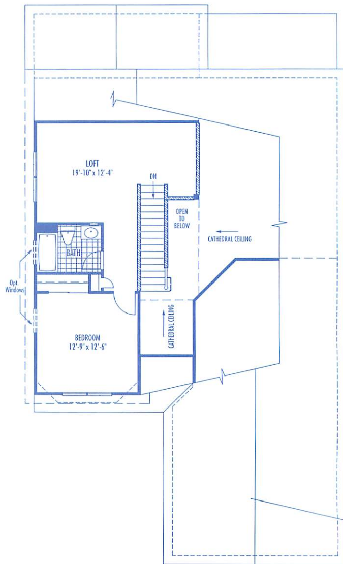
OPT. SECOND FLOOR LOFT • FULL BATH • BEDROOM
