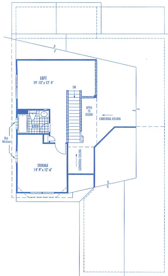
OPT. SECOND FLOOR LOFT • FULL BATH • STORAGE
