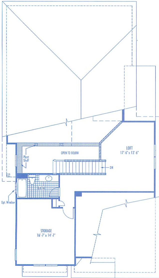
OPT. SECOND FLOOR LOFT • FULL BATH • STORAGE
