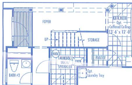
PARTIAL FOYER WITH STAIRS TO OPTIONAL SECOND FLOOR
